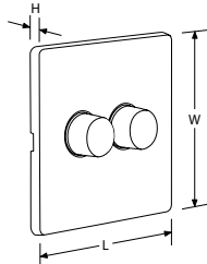
AU-A1BTR2GW (L) 92mm Length (W) 92mm Width (H) 6mm Height (RD) 13mm Recess Depth
