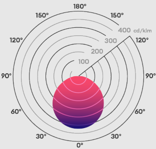
Beam angle: 115°
